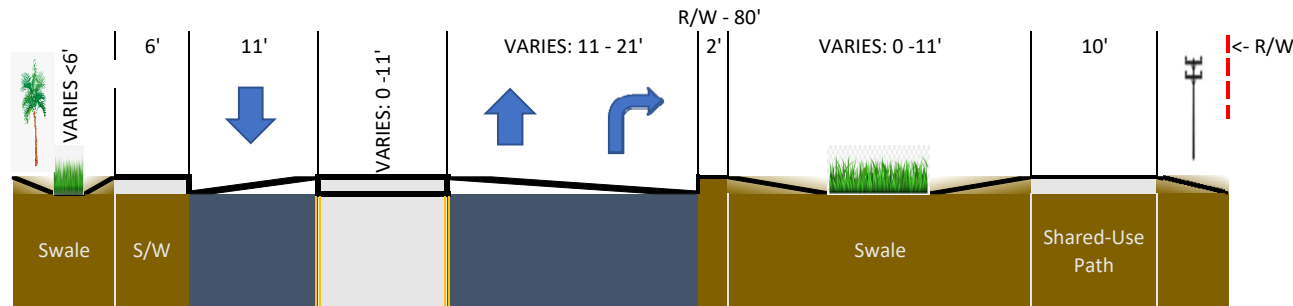
PROPOSED TYPICAL SECTION # 3: Barwick Road from South Sabal Lakes Road to North Sabal Lakes Road
