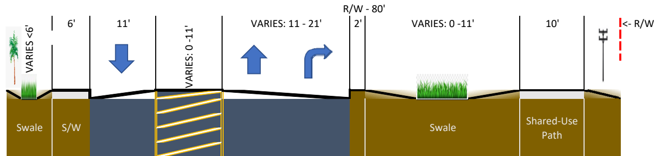
PROPOSED TYPICAL SECTION #2: Barwick Road from North of Canal TO South Sabal Lakes Road
