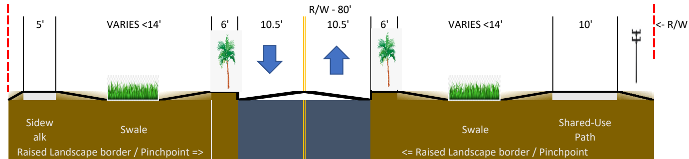
PROPOSED TYPICAL SECTION #1: Barwick Road from North of Lake Ida to North of Canal
